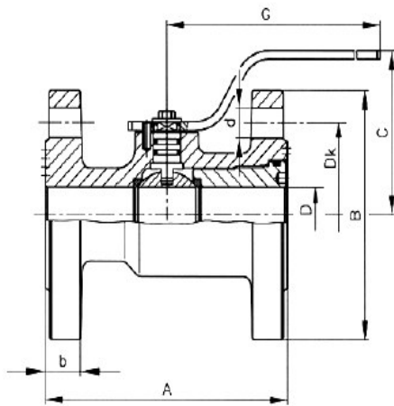
DN 25 - 50
